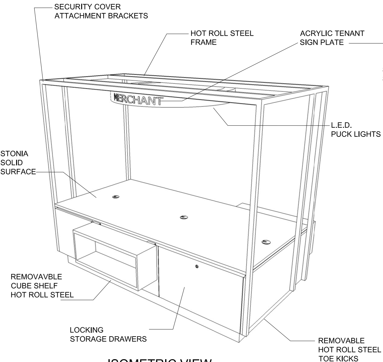
ISOMETRIC VIEW
